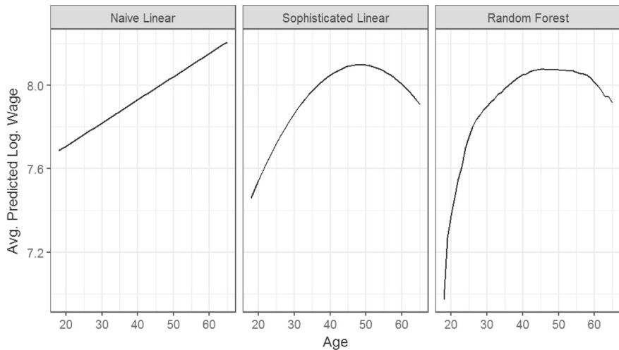
FIGURE 3. – Partial dependence plot for age, computed from three predictive models
