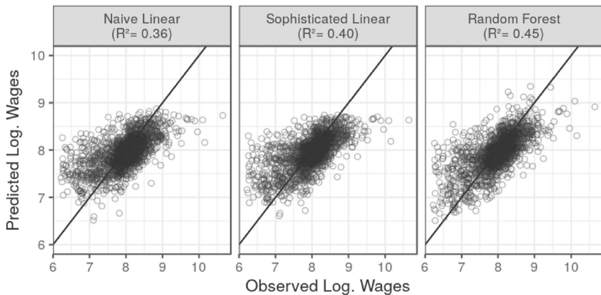
FIGURE 1. – Diagnostics plots, observed vs. predicted wages
